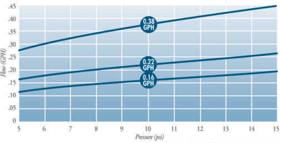
STREAMLINE Flow Rate vs. Pressure
